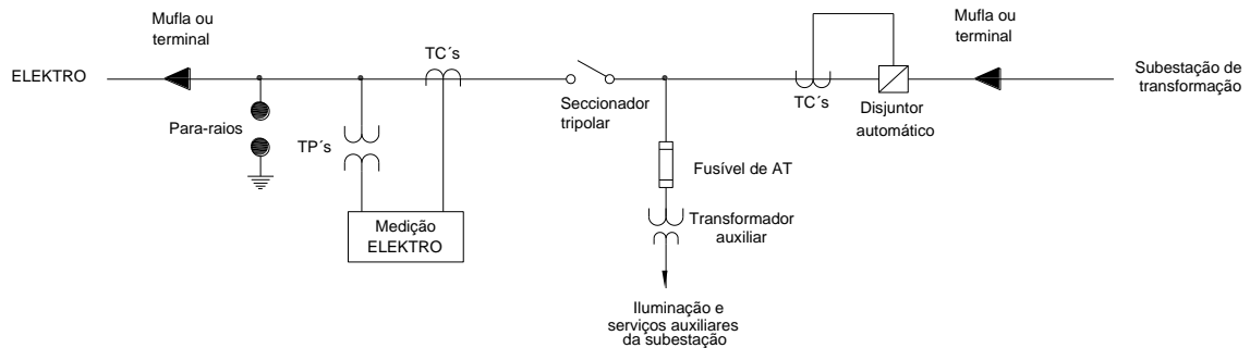
DIAGRAMA UNIFILAR
