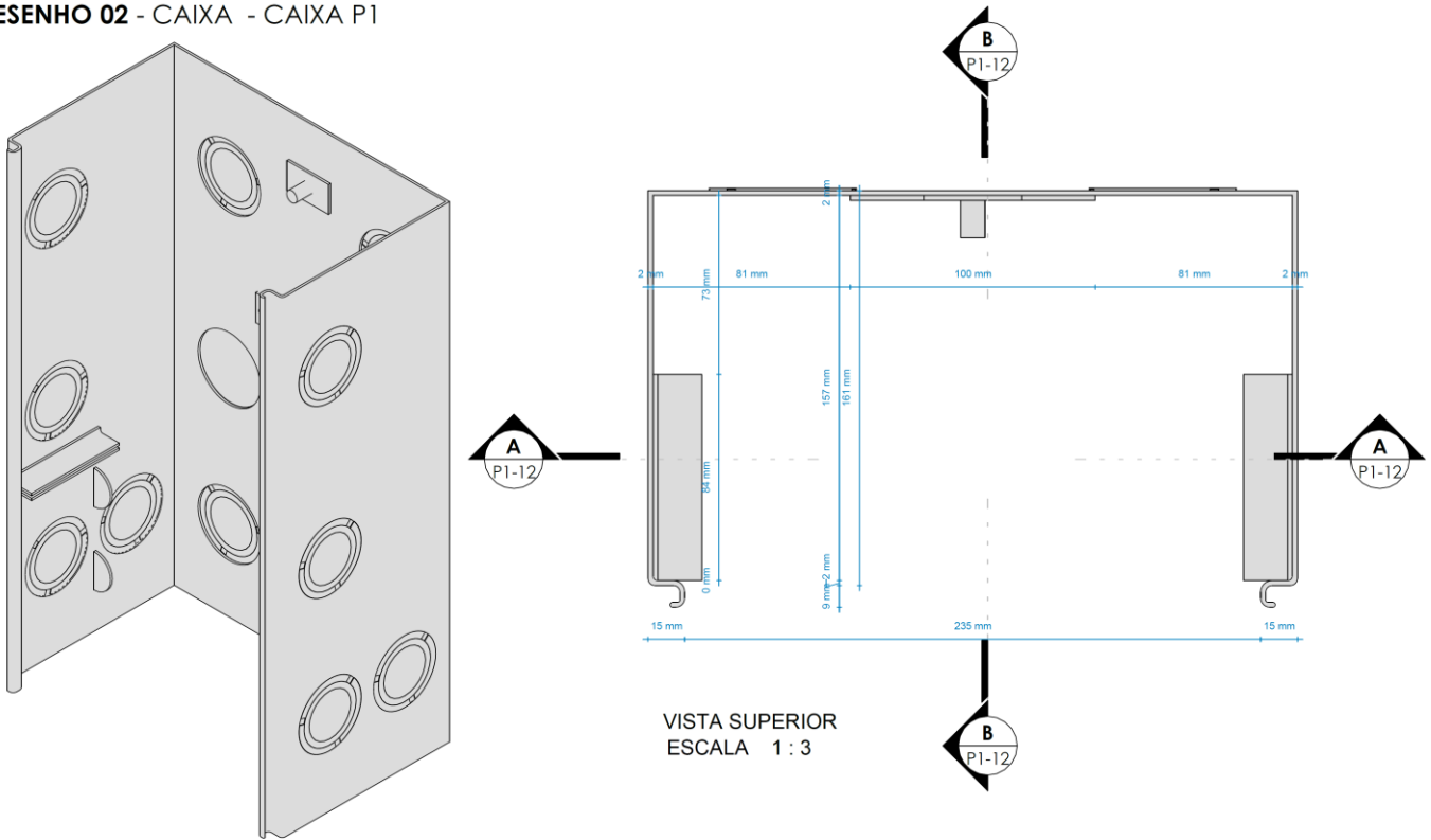
VISTA ORTOGONAL 3D
